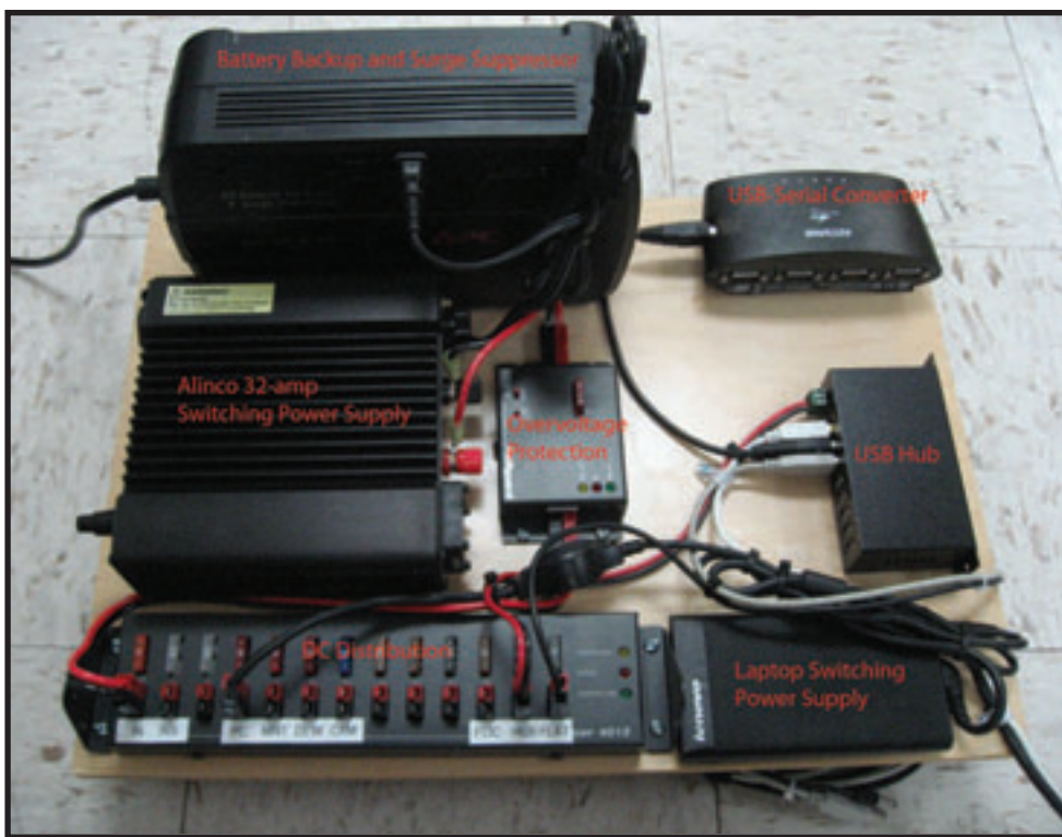
Image 2 - Electronics Board: Uninterruptible 110-volt AC power supply; Alinco DM-330MV 32-amp 13.8-volt switching power supply; Rigrunner DC distribution panel ( www.westmountainradio.com ); USB-serial converter; USB hub; 12-volt power supply for laptop.
